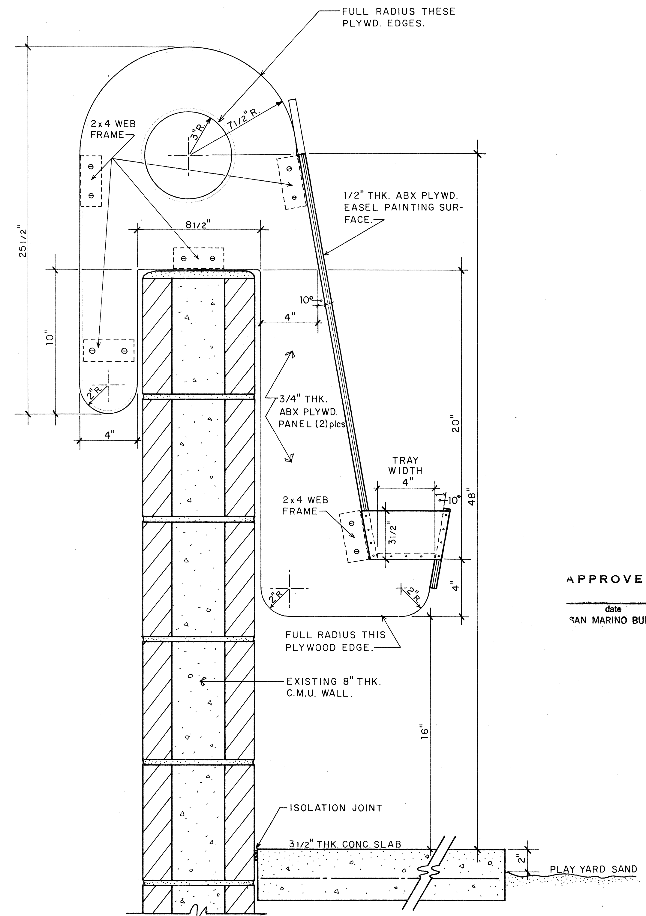
SIDE ELEVATION OF EASEL 3" = 1'-0"
